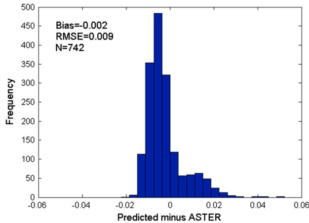
Figure 13. Difference histograms of ASTER BBE and that retrieved by equation (7) from the test data for vertisols in the transition zone.
