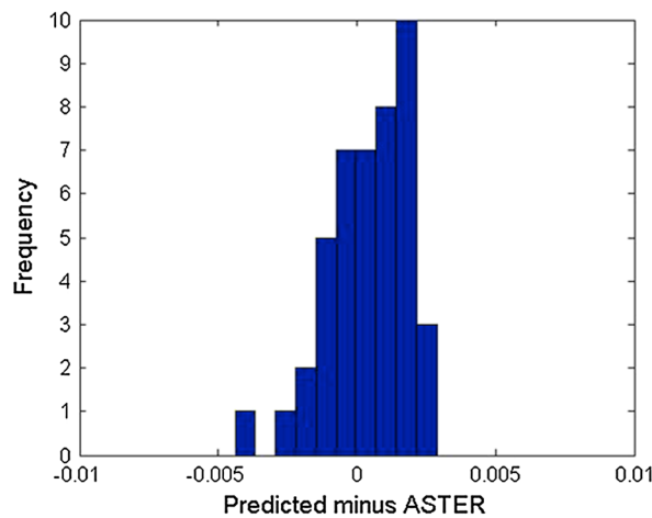
Figure 6. Comparison of ASTER BBE and that predicted by equation 4 from the derivation data for ultisols in bare soil, as well as the histogram of the bias.
