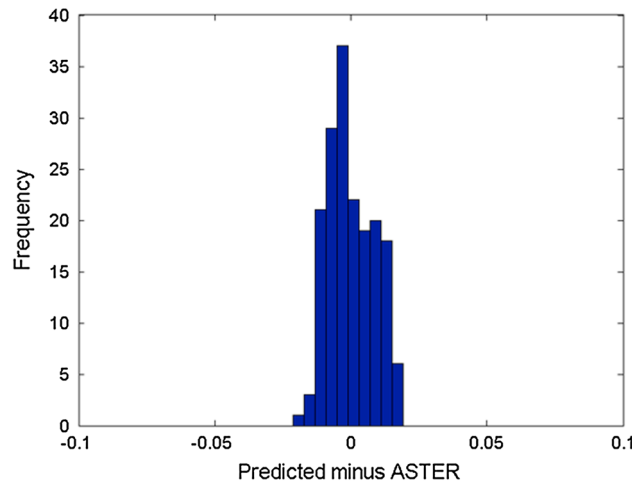
Figure 10. Comparison of ASTER BBE and that predicted by equation 6 from the derivation data for andisols in the transition zone, as well as the histogram of the bias.
