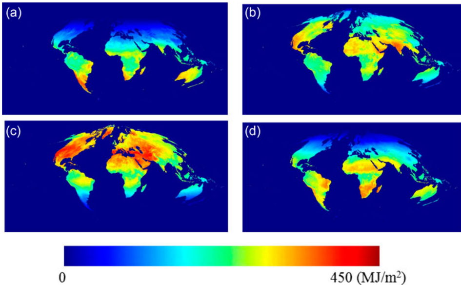
Figure 7. Global land surface monthly integrated incident PAR in 2008 at 5 km spatial resolution calculated from GLASS PAR product in (a) January, (b) April, (c) July, and (d) October.
